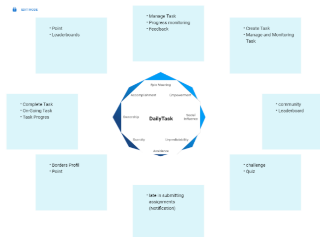
Figure 3. Gamification Elements
